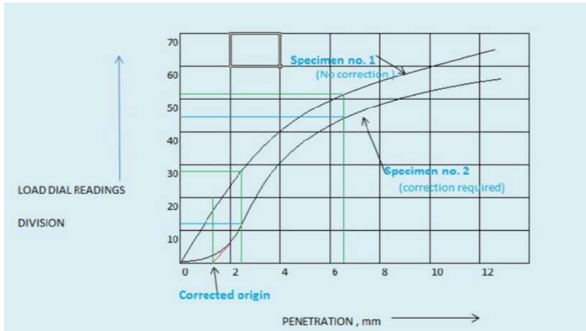
Fig. 4 : Plot of Load versus Settlement
